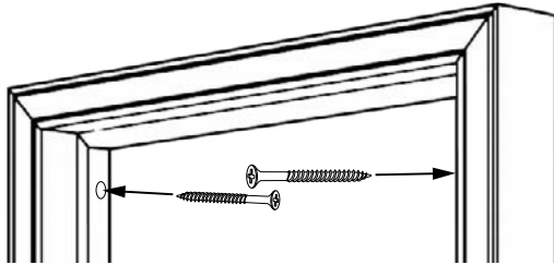
Inside Mount
