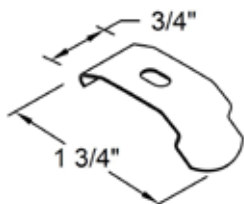
Mounting Clip
