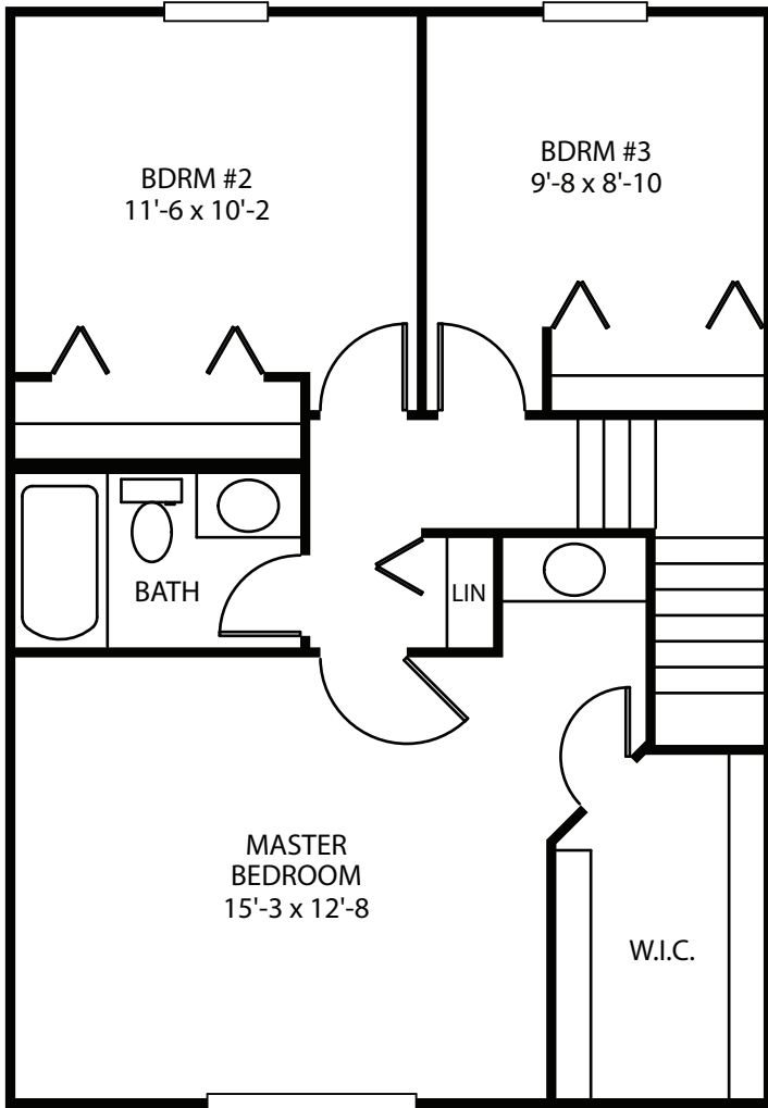
SECOND FLOOR
