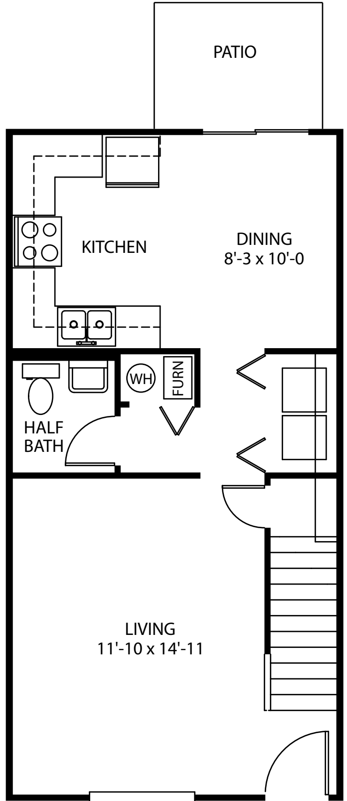
FIRST FLOOR
