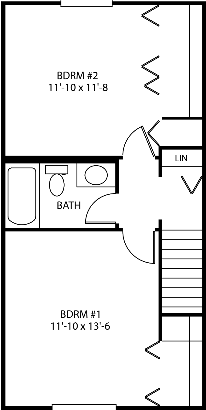
SECOND FLOOR
